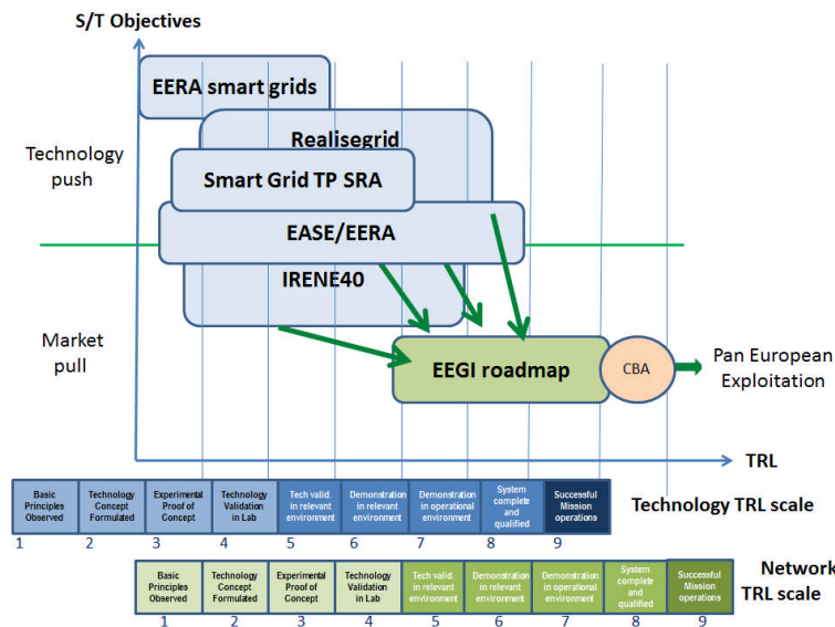
Figure 3 – Positioning of existing roadmaps according to the TRL scale of manufacturers and the TRL scale of network operators.
