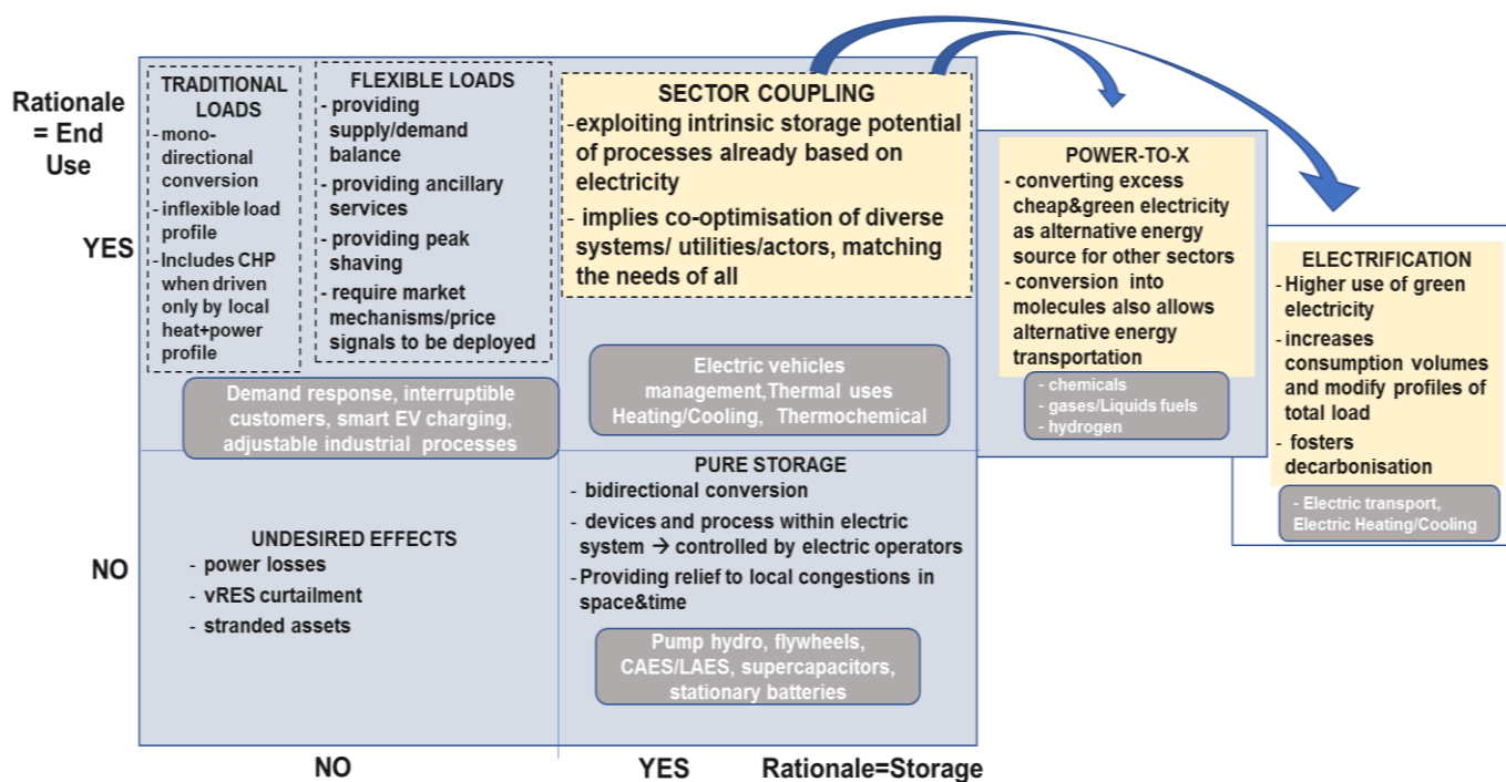
Figure 1.7b) Rationale and characteristics of energy flow processes
