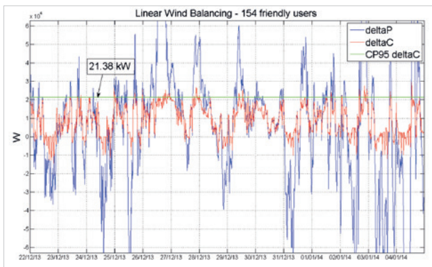
Figure 21: Imbalance (blue) and consumption change (red) of the cluster of households. Green line is the 95th percentile of the limit of the available flexibility
