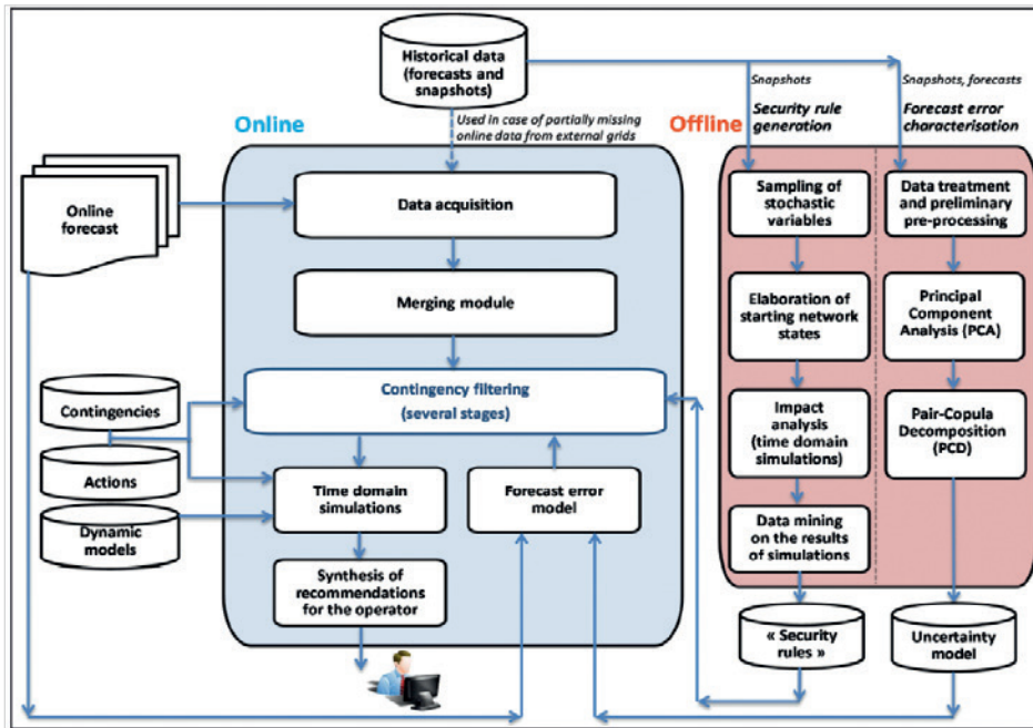
Figure 6: Overall work flow of the iTESLA platform
