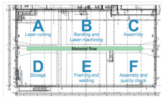
Figure 30: Schematic Overview of Material Flow and Factory Layout
