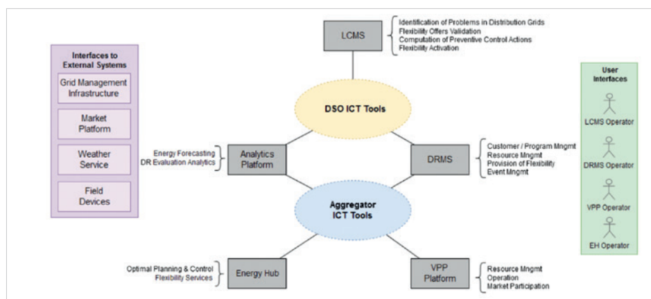
Figure 14: The SmarterEMC2 High Level Conceptual Architecture
