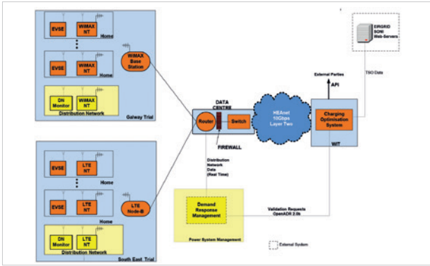
Figure 25: Smart Charging trial Architecture
